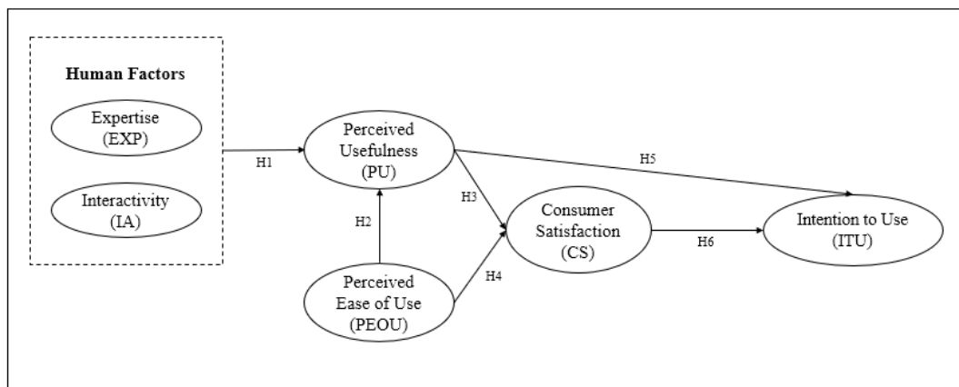
Fig. 1. Research Model
